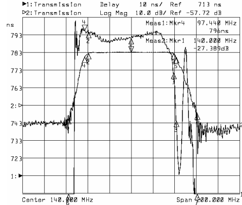
Horizontal: 20MHz/Div Vertical: 20nsec/Div
