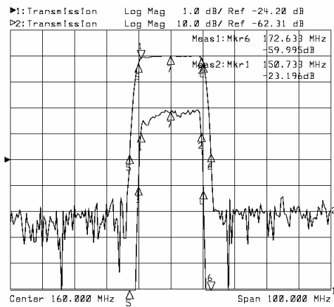
Horizontal: 10MHz/Div Vertical: 10dB/Div
