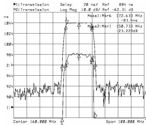
Horizontal: 10MHz/Div Vertical: 20nsec/Div
