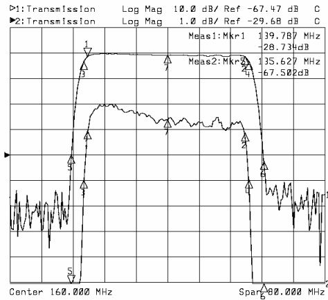
Horizontal: 8MHz/Div Vertical: 10dB/Div
