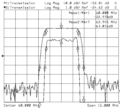
Horizontal: 1.5MHz/Div Vertical: 1dB/Div& 10dB/Div
