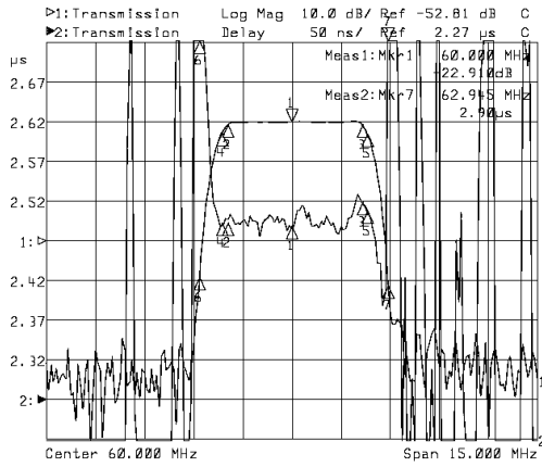
Horizontal: 1.5MHz/Div Vertical: 50nsec/Div& 10dB/Div
