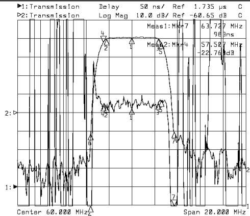
Horizontal: 2.0MHz/Div Vertical: 50nsec/Div & 10 dB/Div
