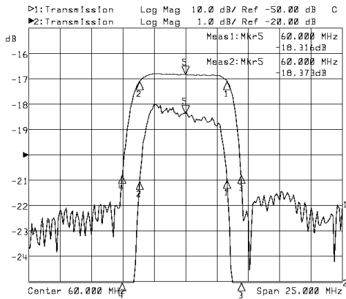
Horizontal: 2.5MHz/Div Vertical: 1dB/Div&10dB/Div
