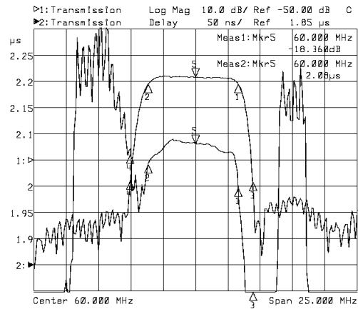
Horizontal: 2.5MHz/Div Vertical: 50ns/Div&10dB/Div
