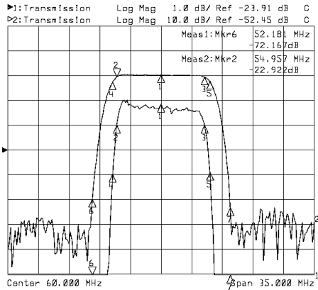
Horizontal: 3.5MHz/Div Vertical: 1dB/Div&10dB/Div
