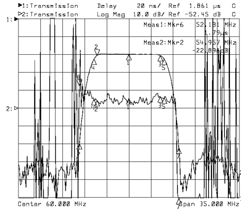
Horizontal: 3.5MHz/Div Vertical: 20nsec/Div&10dB/Div
