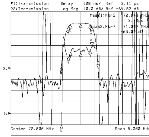
Horizontal: 0.8MHz/Div Vertical: 100ns/Div & 10dB/Div
