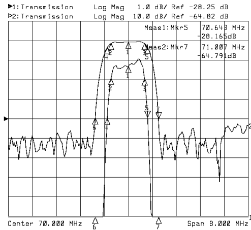
Horizontal: 0.8MHz/Div Vertical: 1dB/Div & 10dB/Div
