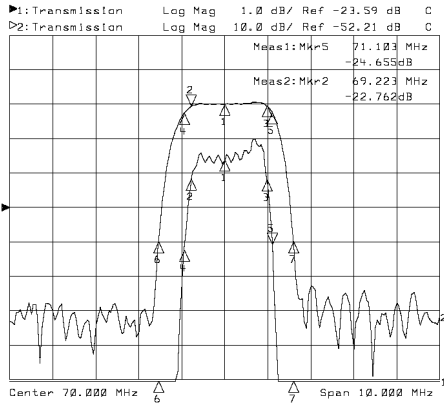
Horizontal: 1.0MHz/Div Vertical: 1dB/Div&10dB/Div
