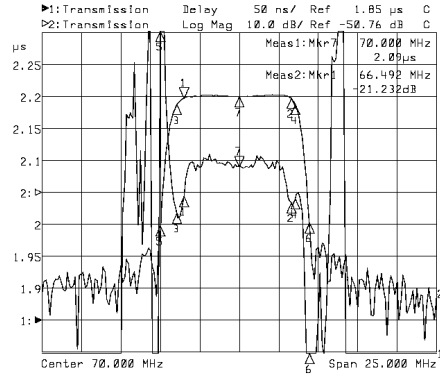
Horizontal: 2.5MHz/Div Vertical: 50nsec/Div & 10dB/Div
