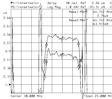
Horizontal: 2.5MHz/Div Vertical: 150nsec/Div & 10dB/Div
