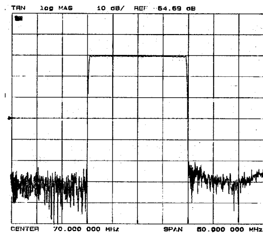
Horizontal: 5MHz/Div Vertical: 10dB/Div
