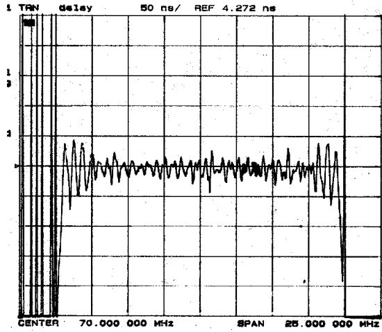
Horizontal: 5MHz/Div Vertical: 50ns/Div
