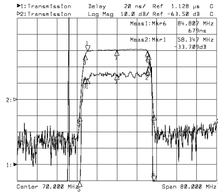
Horizontal: 8MHz/Div Vertical: 20nsec/Div&10dB/Div
