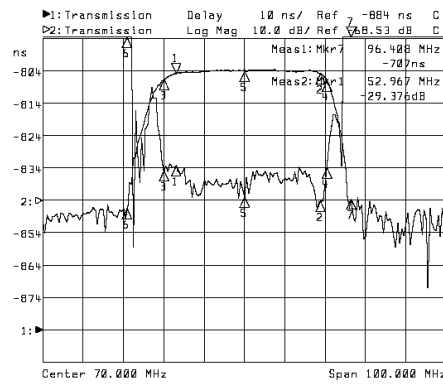
Horizontal: 10MHz/Div Vertical: 10nsec/Div&10dB/Div
