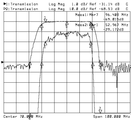
Horizontal: 10MHz/Div Vertical: 1dB/Div&10dB/Div
