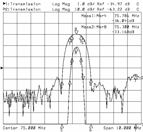
Horizontal: 1MHz/Div Vertical: 10dB/Div
