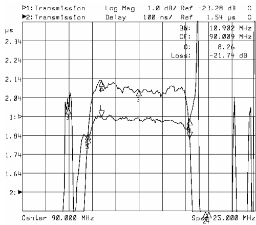
Horizontal: 2.5MHz/Div Vertical: 100nsec/Div
