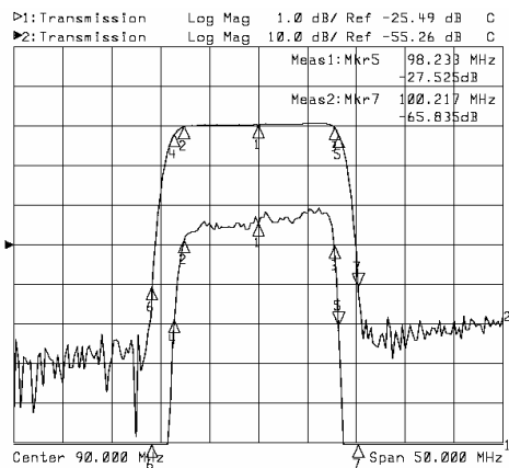
Horizontal: 5MHz/Div Vertical: 10dB/Div
