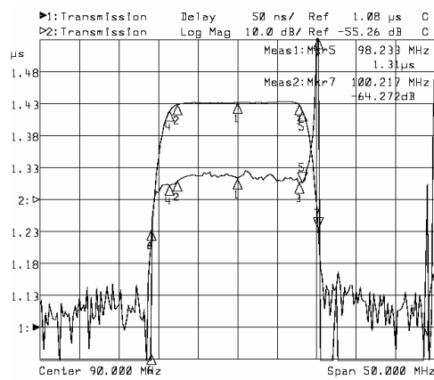
Horizontal: 5MHz/Div Vertical: 50nsec/Div
