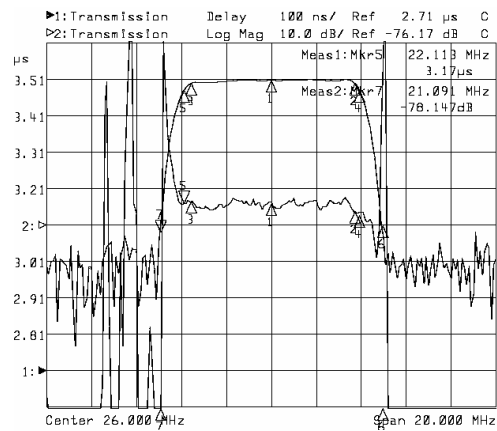
Horizontal: 2.0MHz/Div Vertical: 100ns/Div
