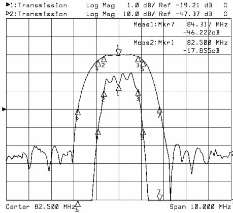
Horizontal: 1.5MHz/Div Vertical: 10dB/Div
