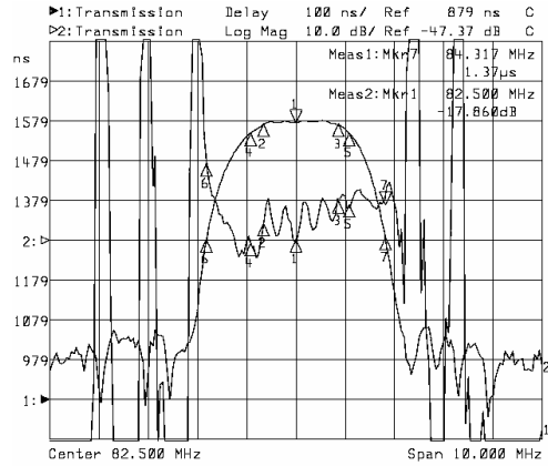
Horizontal: 1.5MHz/Div Vertical: 50nsec/Div
