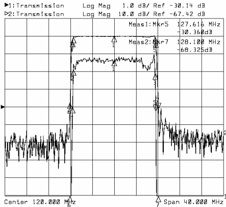
Horizontal: 4MHz/Div Vertical: 10dB/Div
