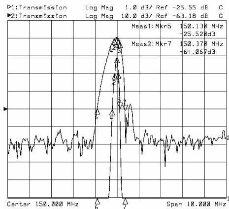
Horizontal: 0.8MHz/Div Vertical: 10dB/Div
