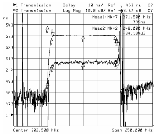
Horizontal: 25MHz/Div Vertical: 10ns/Div
