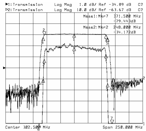
Horizontal: 25MHz/Div Vertical: 10dB/Div
